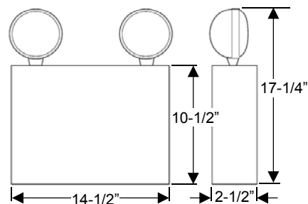
50 Watt Capacity
