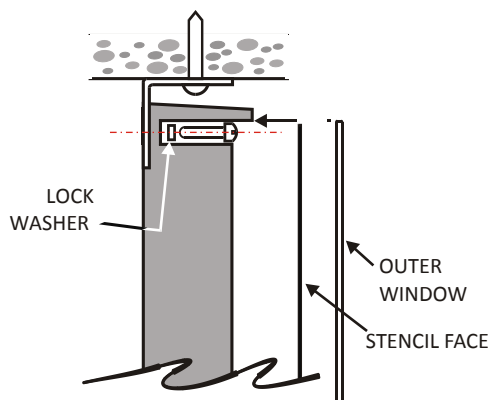
TOP MOUNT
