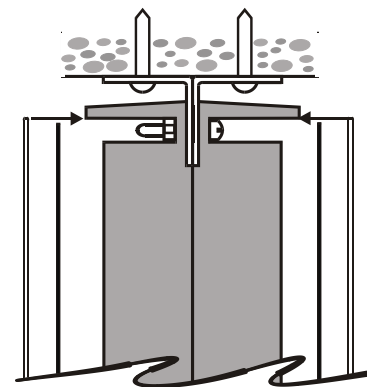
DOUBLE FACE
