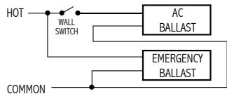
Primary circuit only. Lamp leads not shown.
