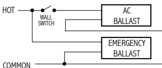
Primary circuit only. Lamp leads not shown.
