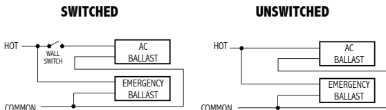
Primary circuit only. Lamp leads not shown.
