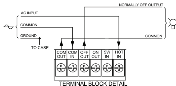
Diagram 4. SWITCHED LOADS
