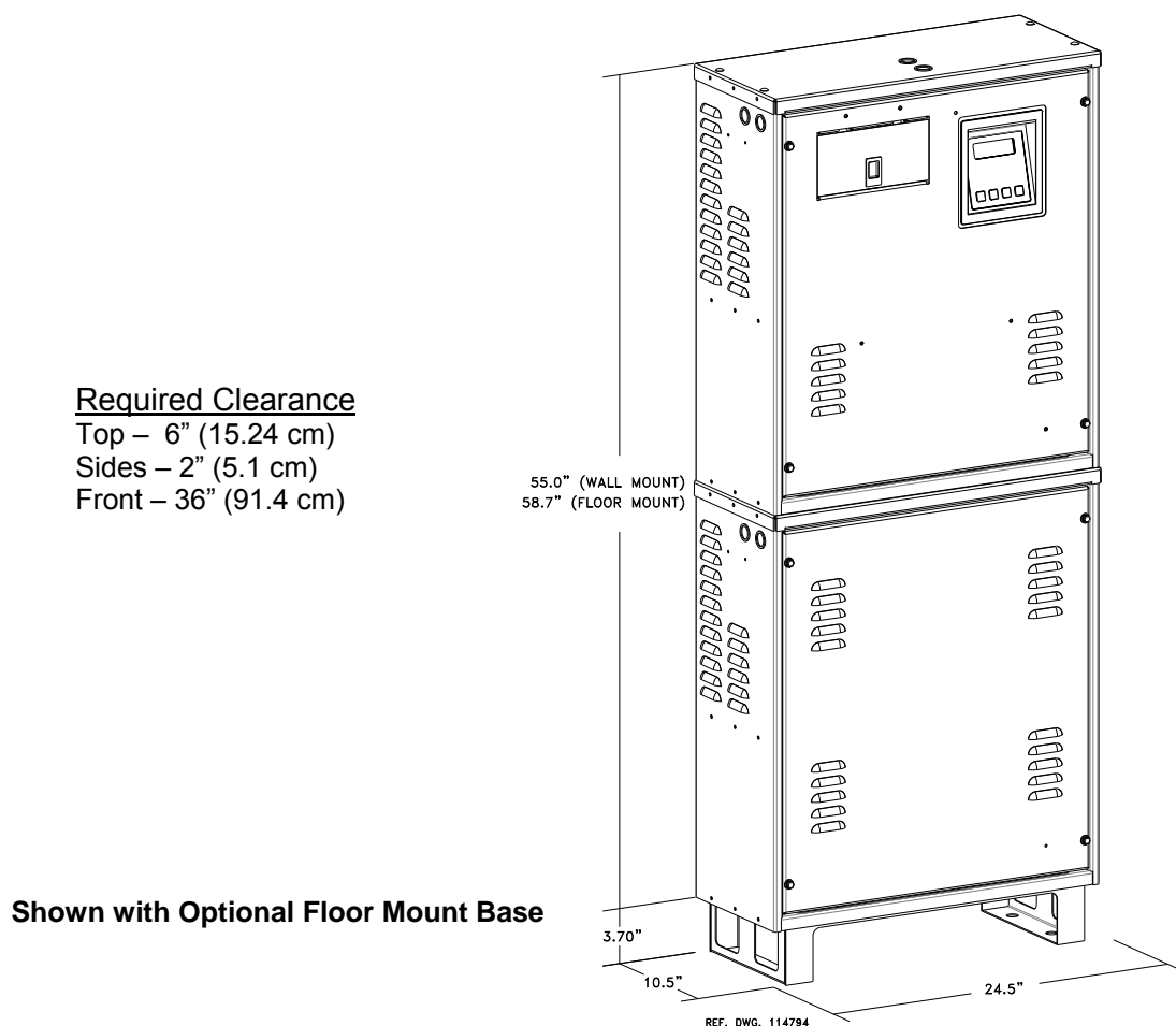
Figure 3.3 2800W System Dimensions
