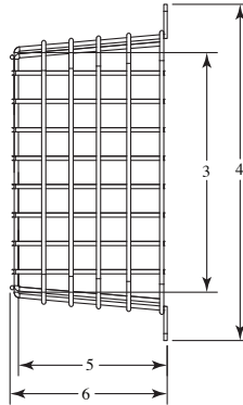
WG-STI-9641, WG-STI-9644, WG-STI-9645 SIDE VIEW
